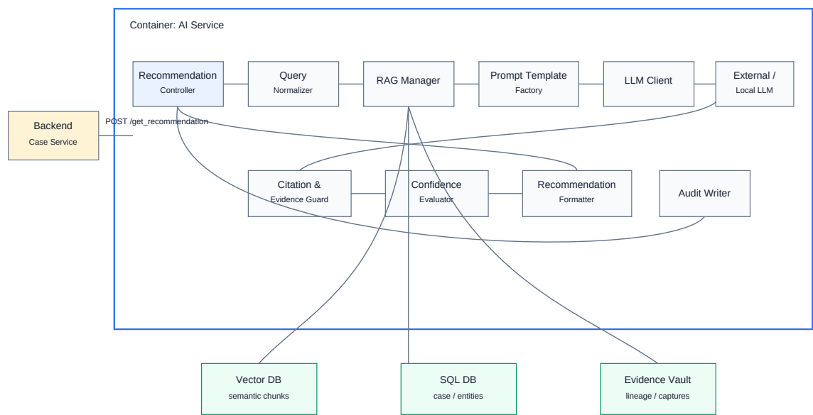
C3 components match the Sequence Diagram one-to-one
